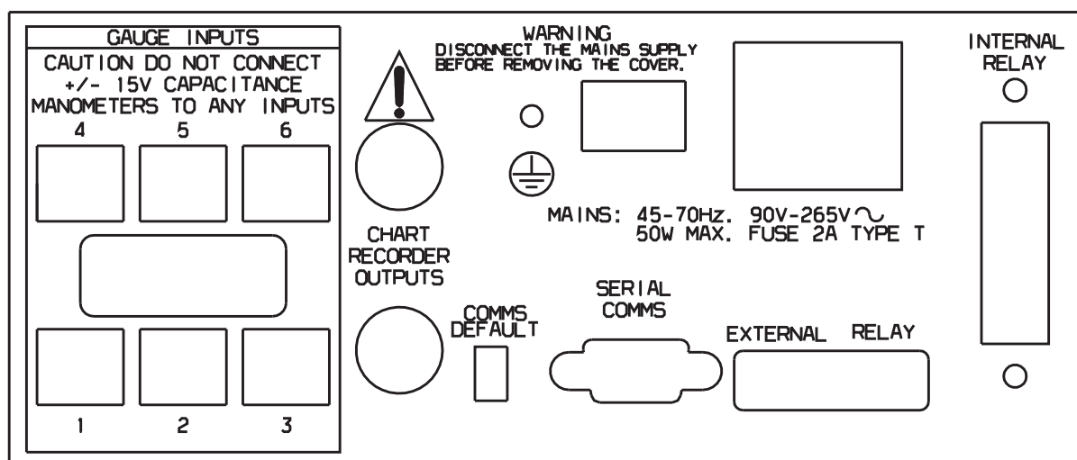
Figure 1 - Rear Panel of the AGC
