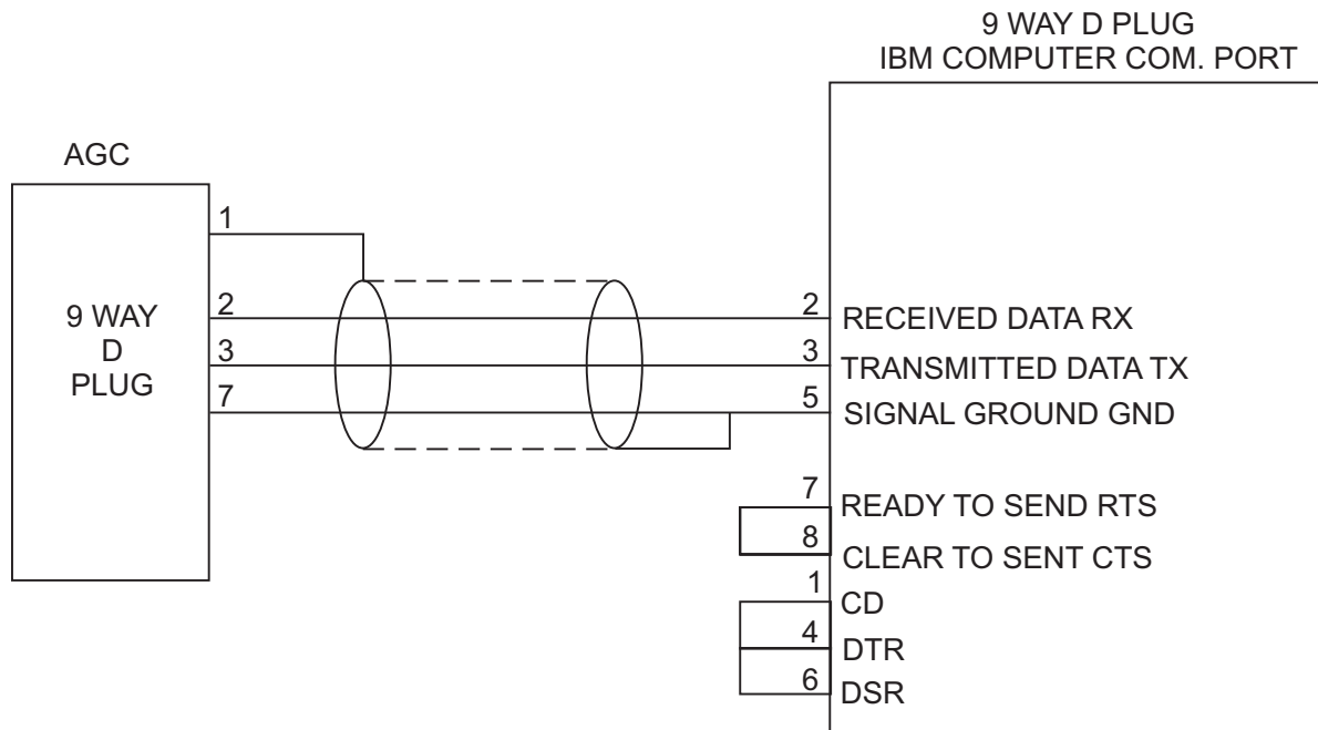
Figure 3 - AGC/IBM Computer Interface
